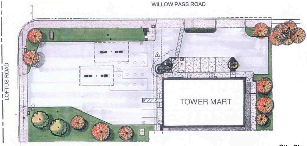
Site Plan
