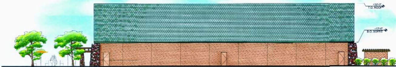
WEST ELEVATION OF WEST BUILDING SCALE: 1/8" = 1'-0"
